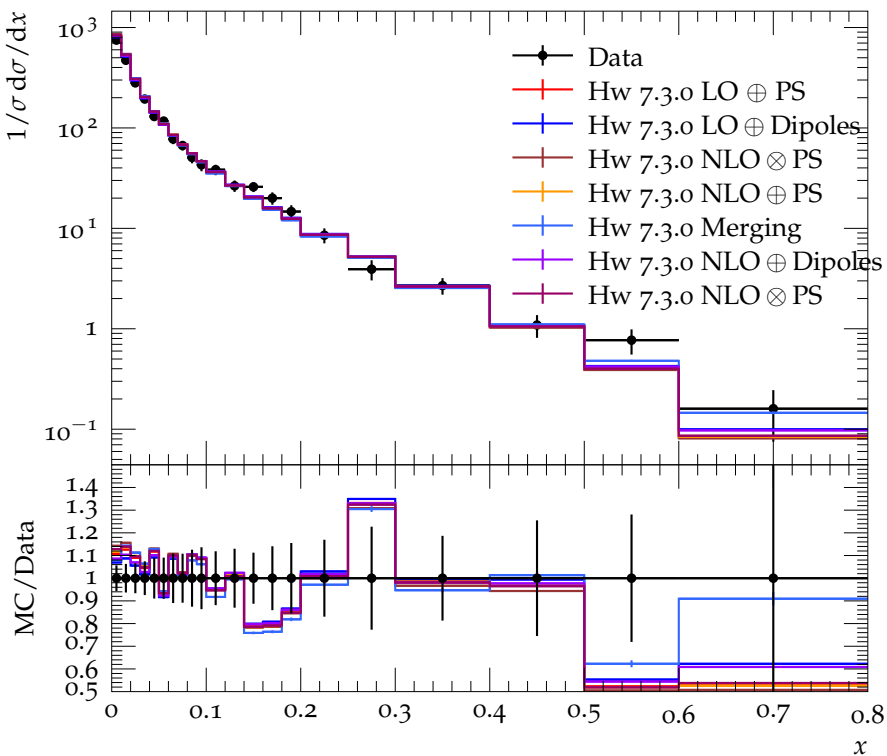
Scaled momentum at 172 GeV
