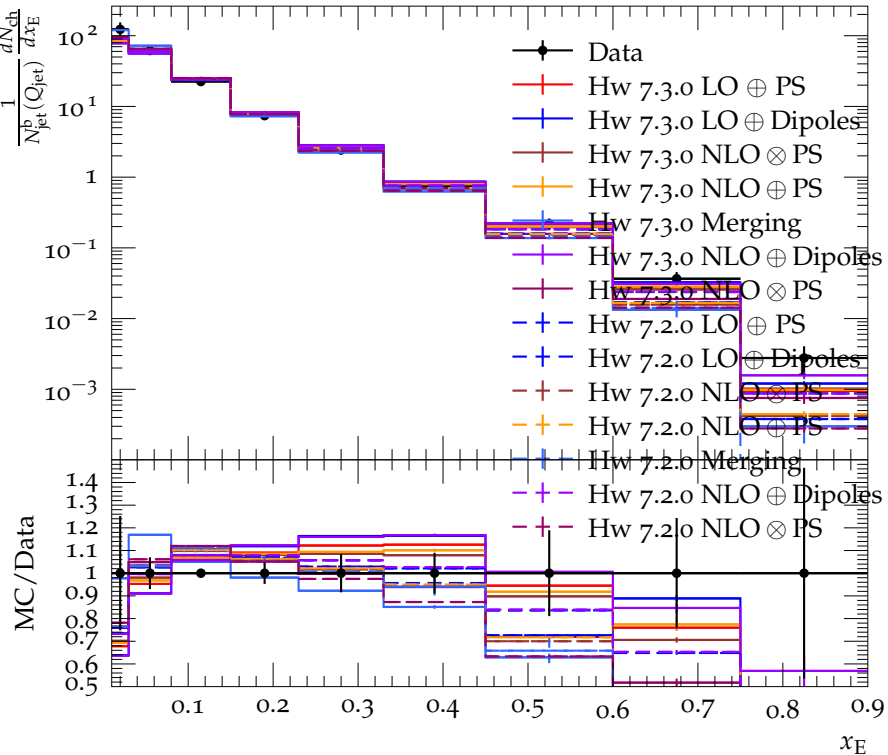
b durham jet fragmentation, Q_{\text{jet}} = 9.0 - 19.0 GeV
