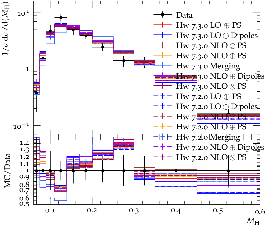
Heavy hemisphere mass, M_H , at 133 GeV
