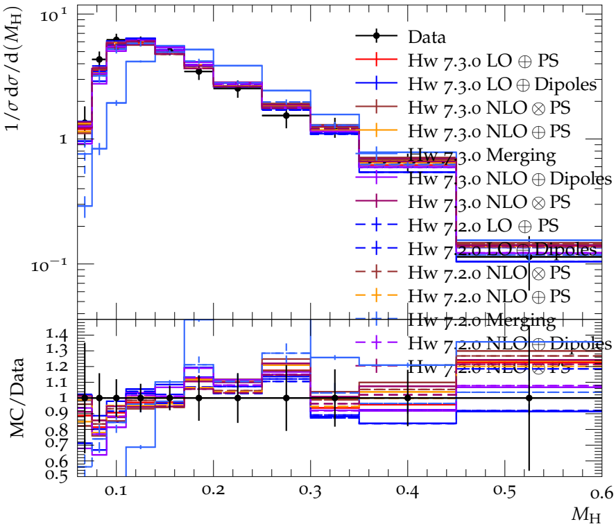
Heavy hemisphere mass, M_H , at 177 (161–183) GeV
