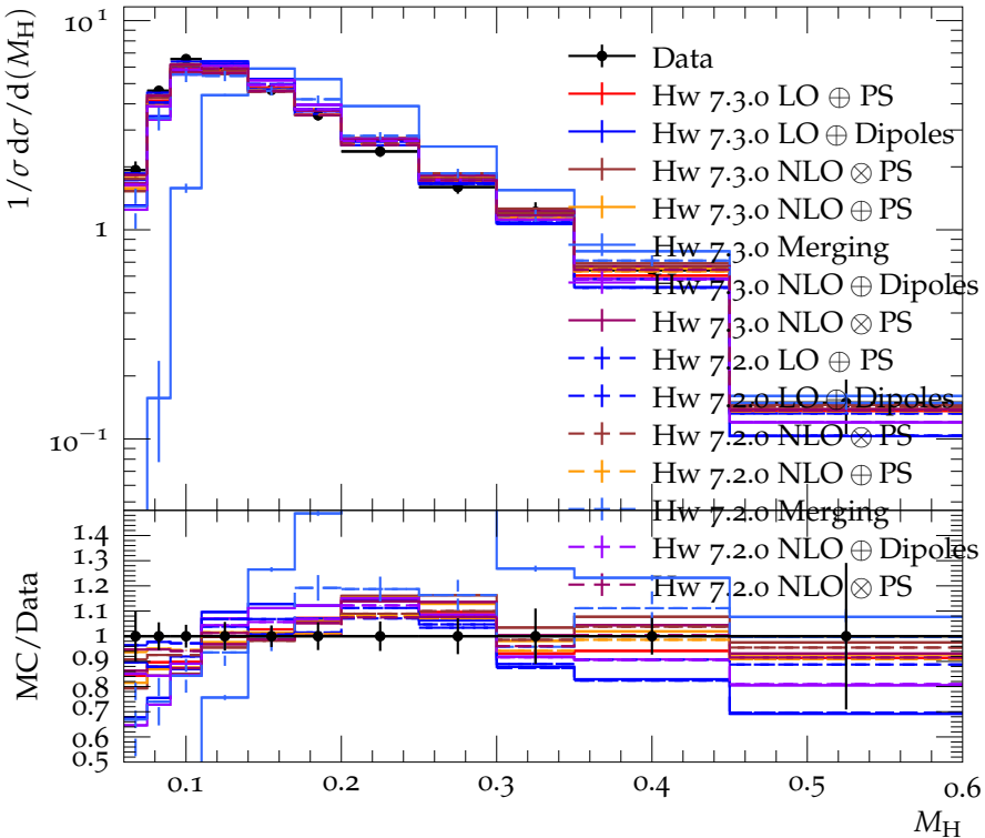
Heavy hemisphere mass, M_H , at 197 (189–209) GeV
