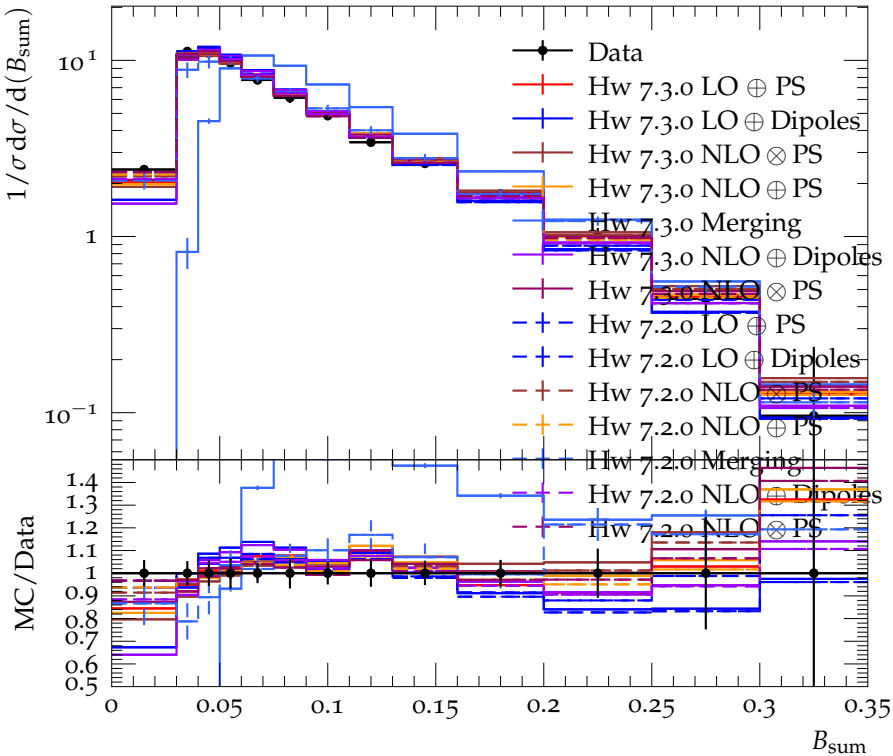
Total hemisphere broadening, B_{\text{sum}} , at 197 (189–209) GeV
