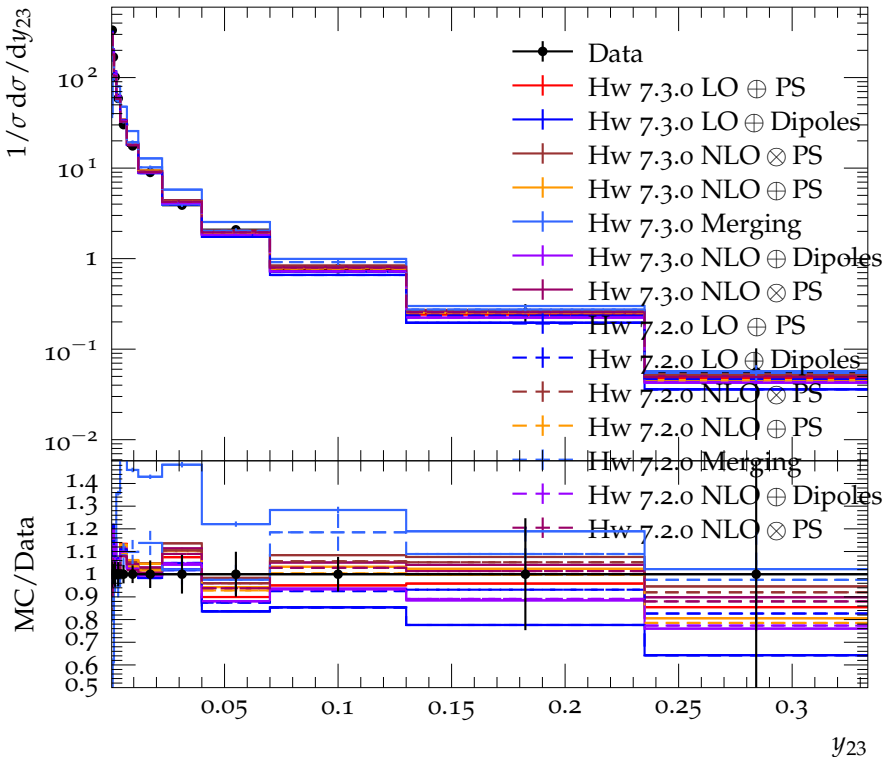
Durham jet 2 \rightarrow 3 transition parameter, y_{23} , at 197 (189–209) GeV
