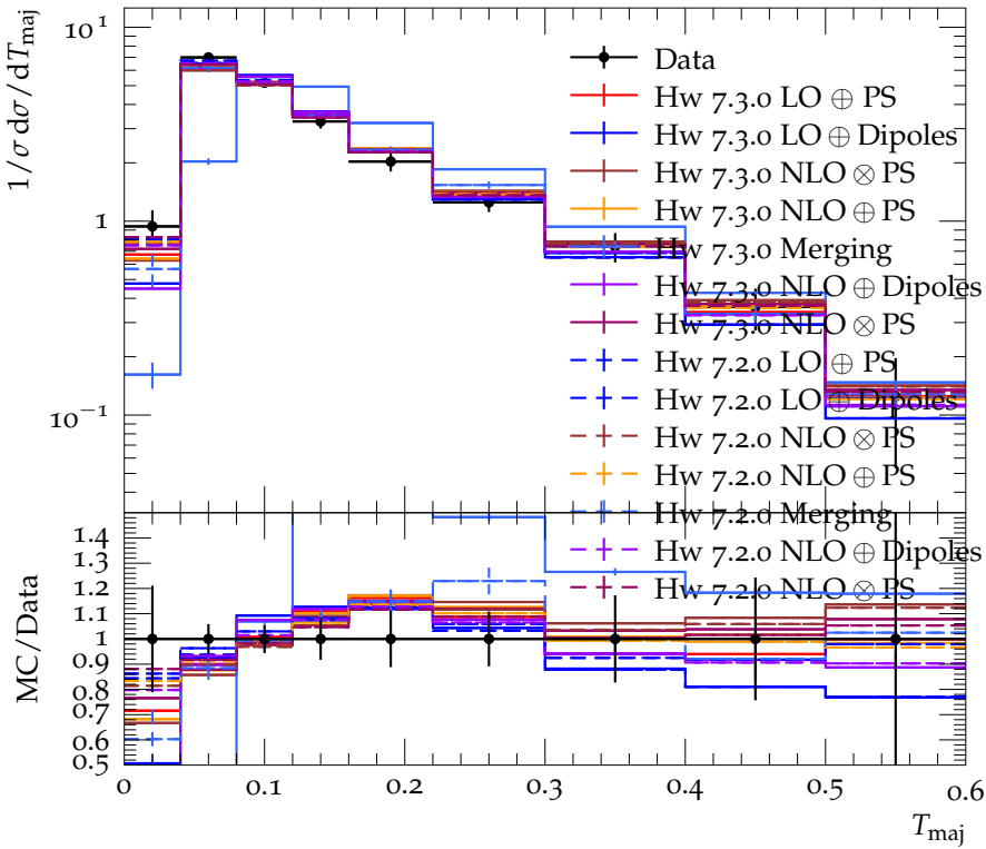
Thrust major, T_{\text{maj}} , at 177 (161–183) GeV
