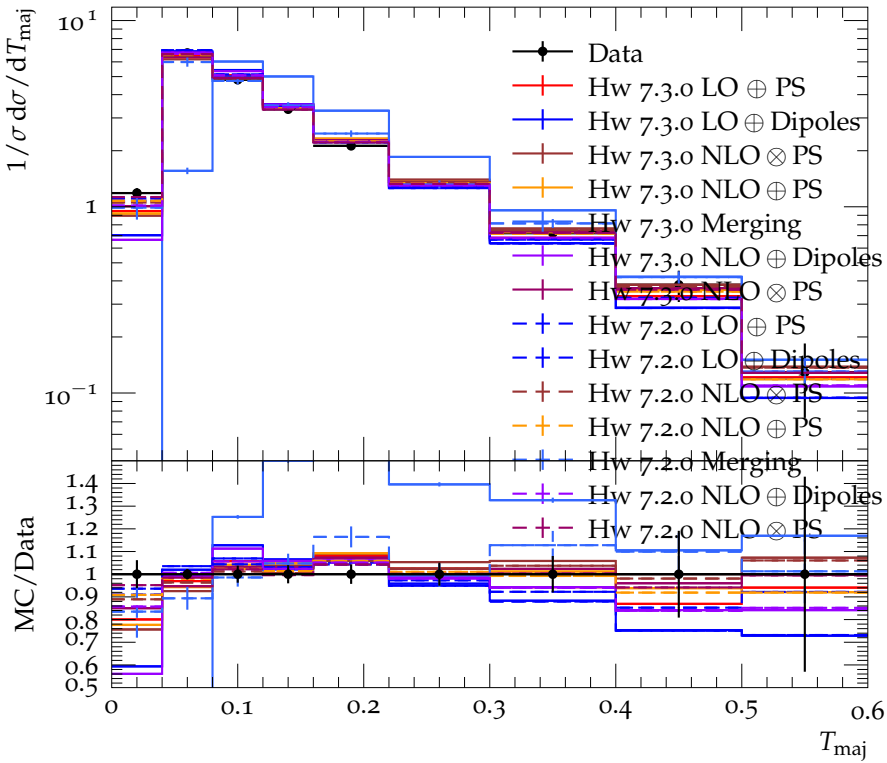
Thrust major, T_{\text{maj}} , at 197 (189–209) GeV
