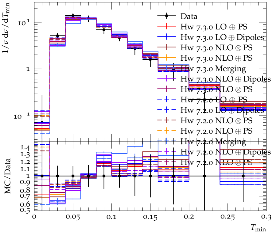
Thrust minor, T_{\min} , at 133 GeV
