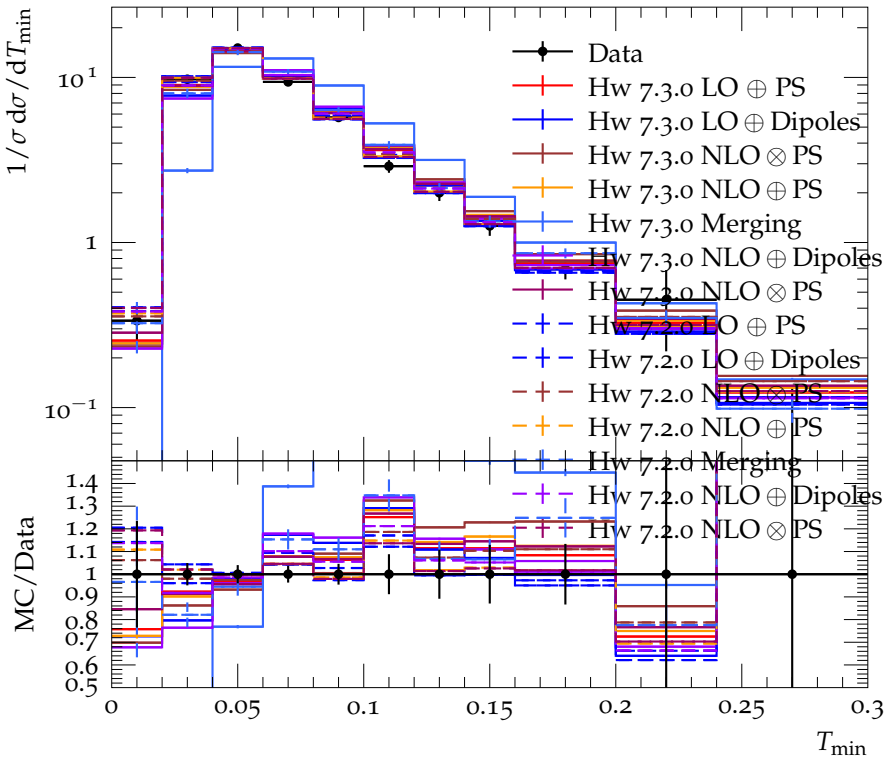
Thrust minor, T_{\min} , at 197 (189–209) GeV
