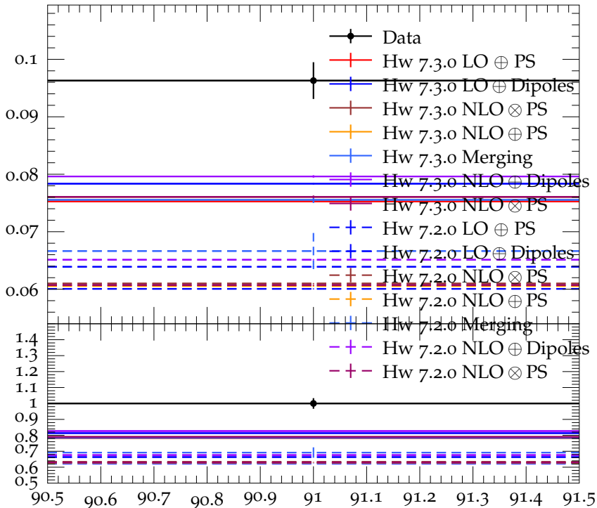
Mean \phi(1020) multiplicity
