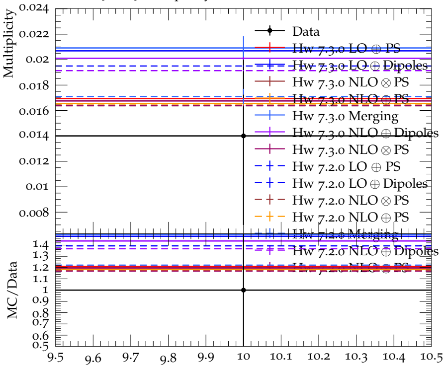
Mean \Sigma_c^{++}, \Sigma_c^0 multiplicity
