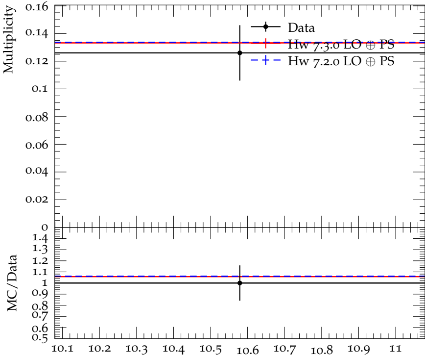
Mean D_s^{*\pm} multiplicity
