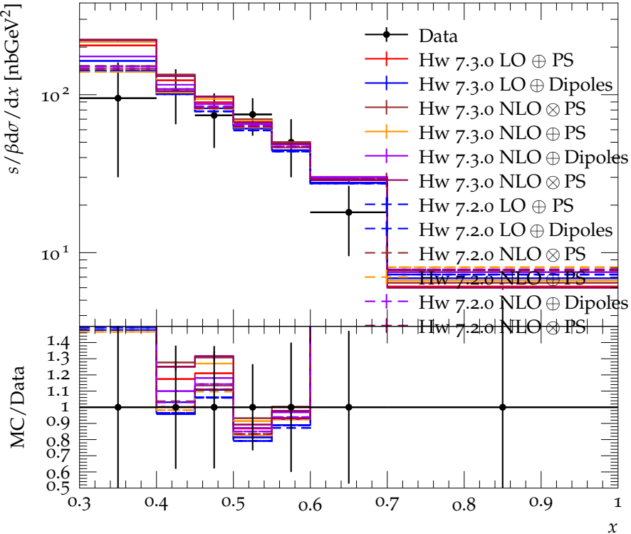
K_S^0 scaled momentum spectrum at E_{\text{CMS}} = 3.63 GeV
