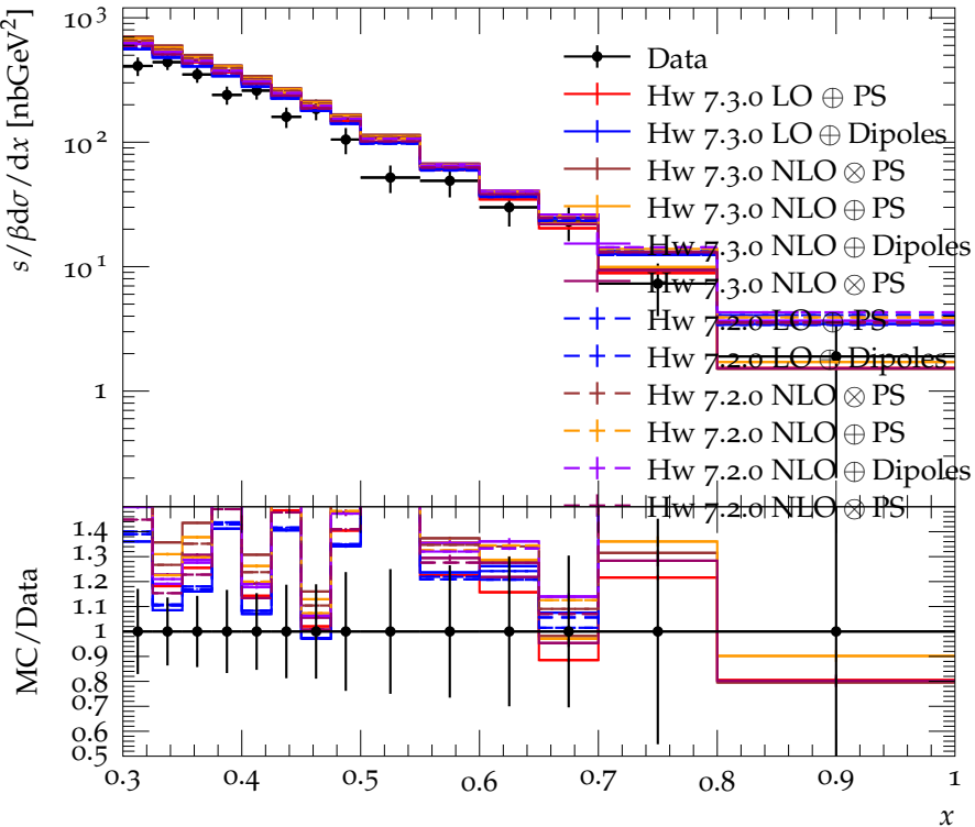
K_S^0 scaled momentum spectrum at E_{\text{CMS}} = 4.5 GeV
