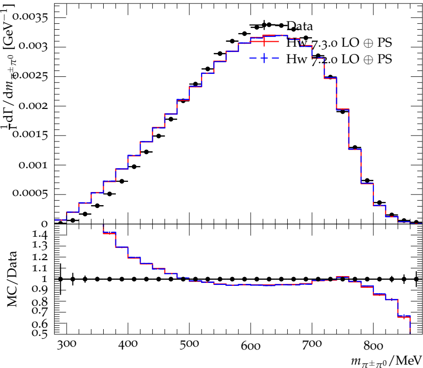
Mass distribution for \pi^\pm\pi^0 in \phi \rightarrow \pi^+\pi^-\pi^0
