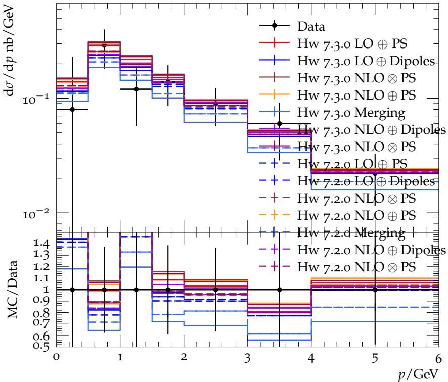
K^0, \bar{K}^0 momentum spectrum for E_{\text{CMS}} = 14 GeV
