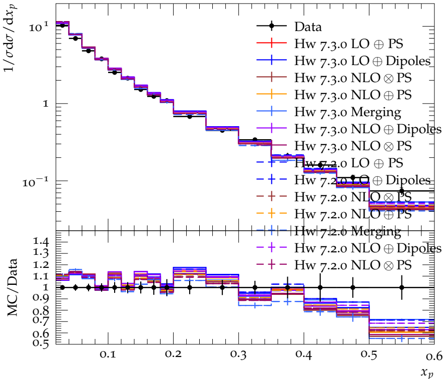
Scaled momentum distribution ( \sqrt{s} = 30 \rightarrow 31.6 GeV)
