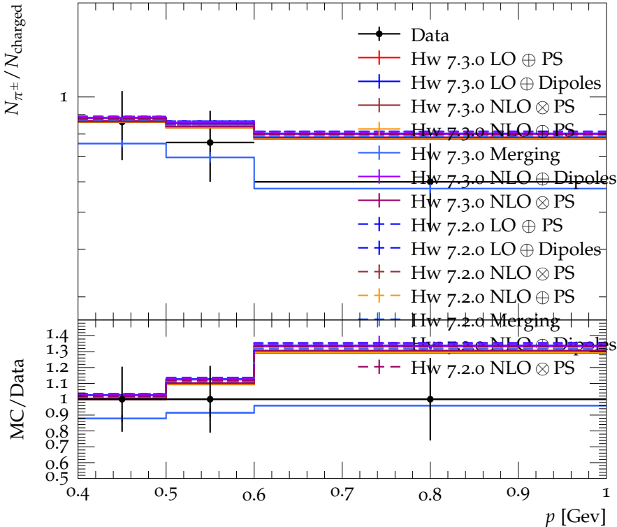
Ratio of \pi^\pm to charged particles at 12 GeV
