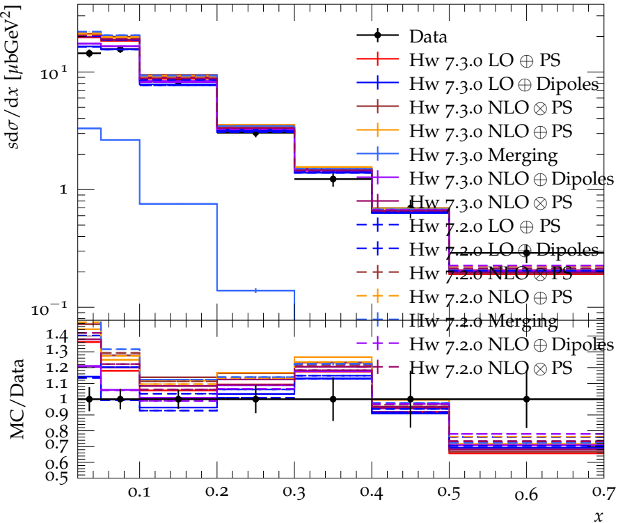
Charged particle scaled momentum, E_{\text{CMS}} = 12 \text{ GeV}
