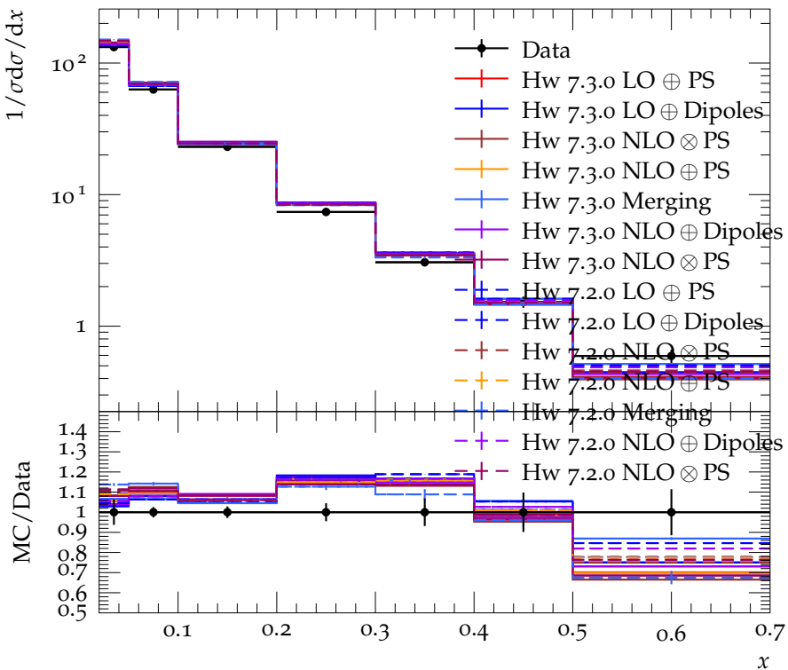
Charged particle scaled momentum, E_{\text{CMS}} = 30 \text{ GeV}
