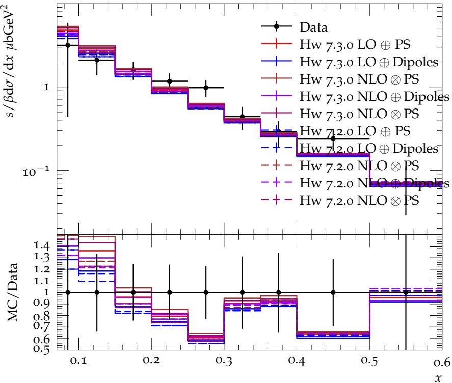
K^0, \bar{K}^0 scaled momentum spectrum for E_{\text{CMS}} = 14 GeV
