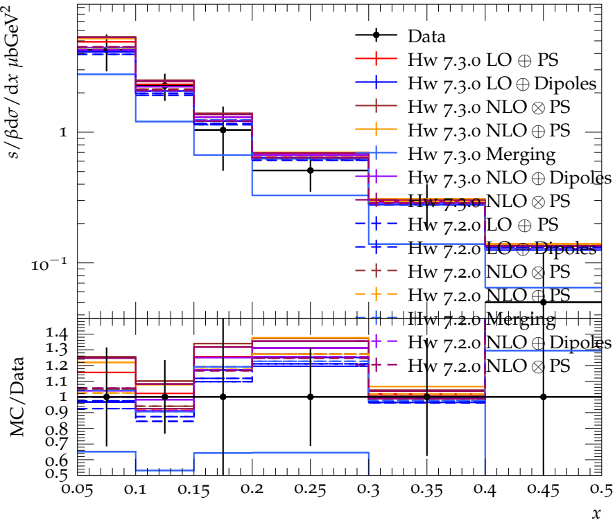
K^0, \bar{K}^0 scaled momentum spectrum for E_{\text{CMS}} = 22 GeV
