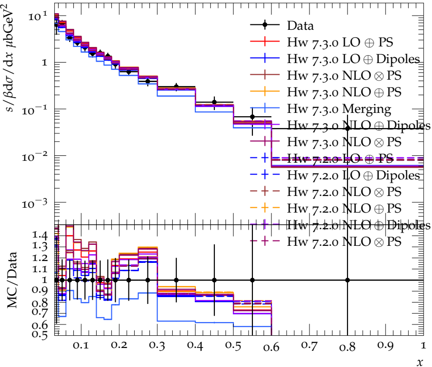
K^0, \bar{K}^0 scaled momentum spectrum for E_{\text{CMS}} = 34 GeV
