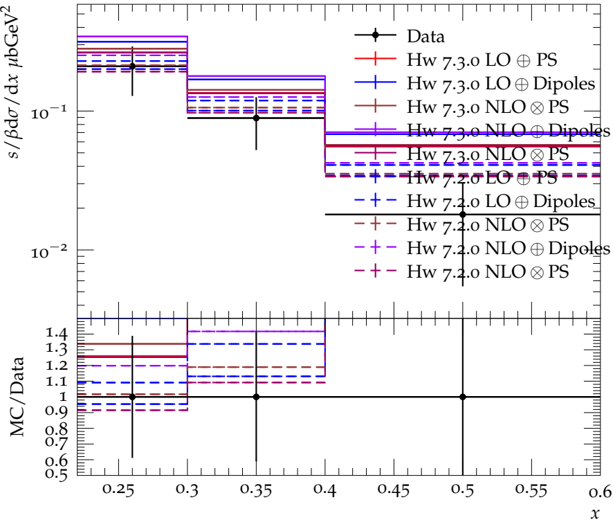
\Lambda^0, \bar{\Lambda}^0 scaled momentum spectrum for E_{\text{CMS}} = 14 GeV
