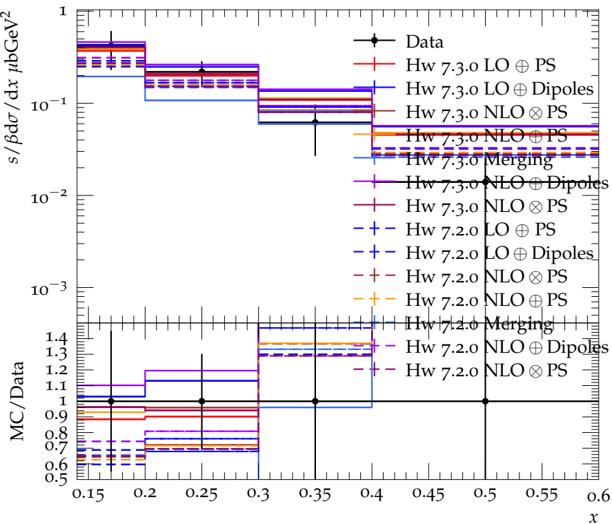
\Lambda^0, \bar{\Lambda}^0 scaled momentum spectrum for E_{\text{CMS}} = 22 GeV
