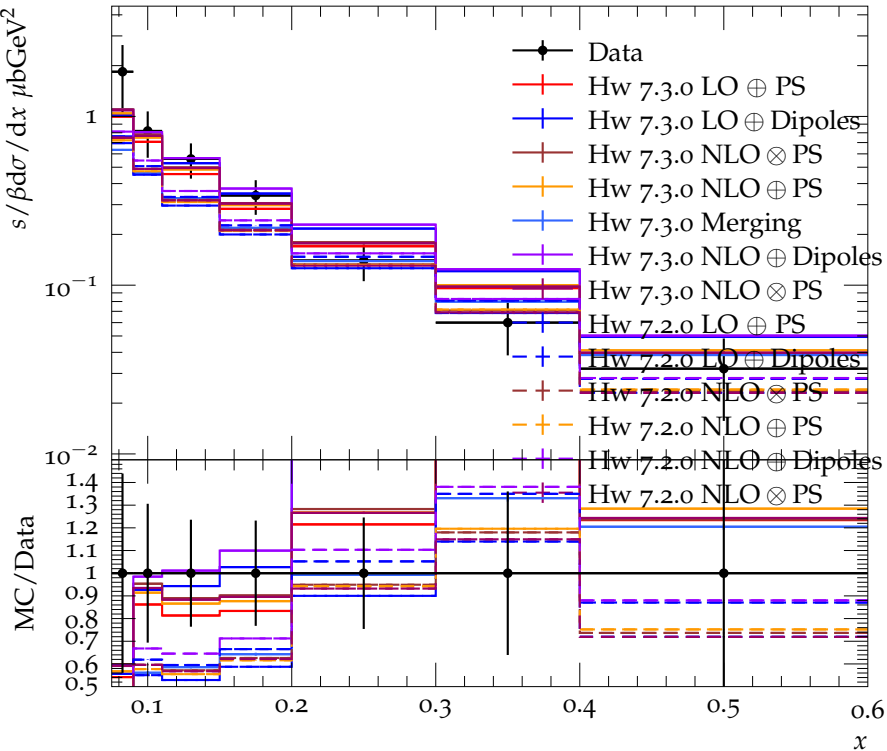
\Lambda^0, \bar{\Lambda}^0 scaled momentum spectrum for E_{\text{CMS}} = 34 GeV
