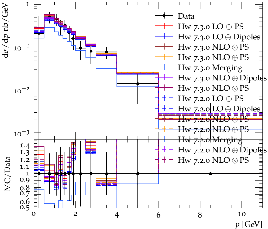
K^0, \bar{K}^0 momentum spectrum for E_{\text{CMS}} = 22 GeV
