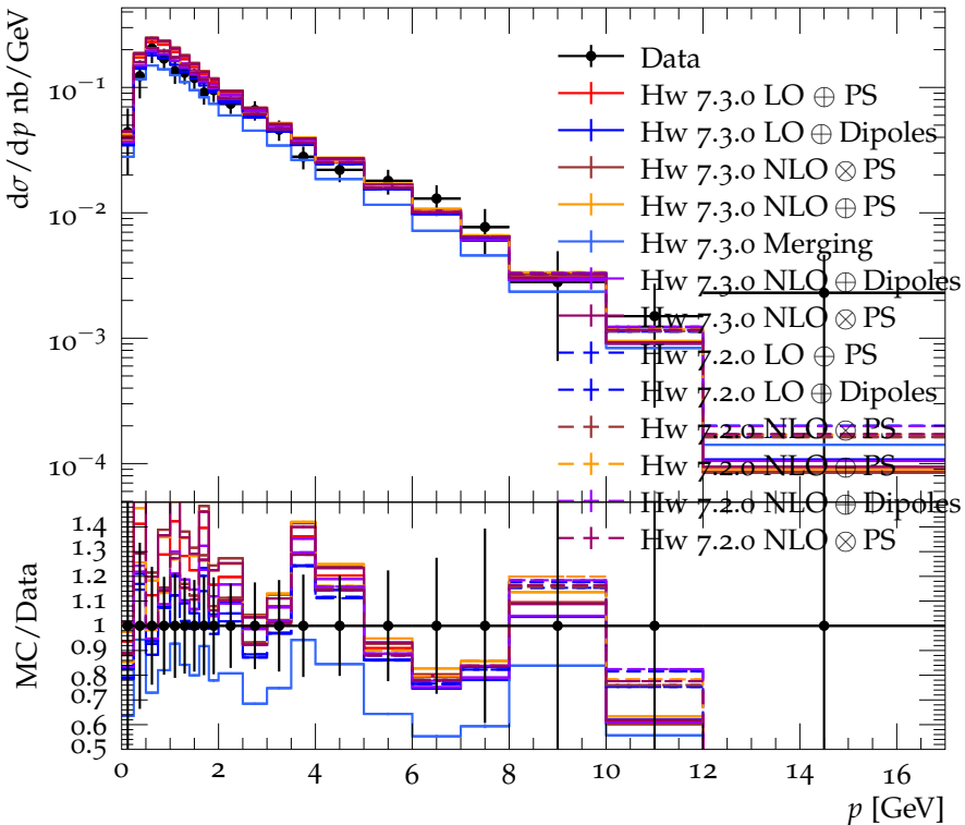
K^0, \bar{K}^0 momentum spectrum for E_{\text{CMS}} = 34 GeV
