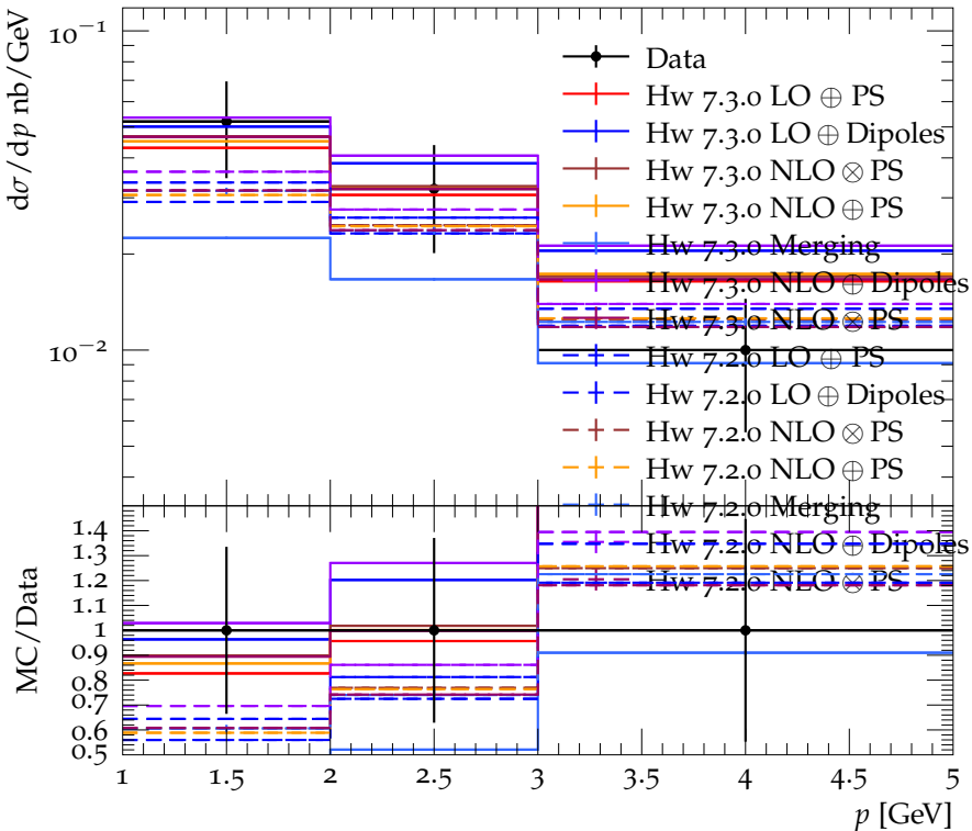
\Lambda^0, \bar{\Lambda}^0 momentum spectrum for E_{\text{CMS}} = 22 GeV
