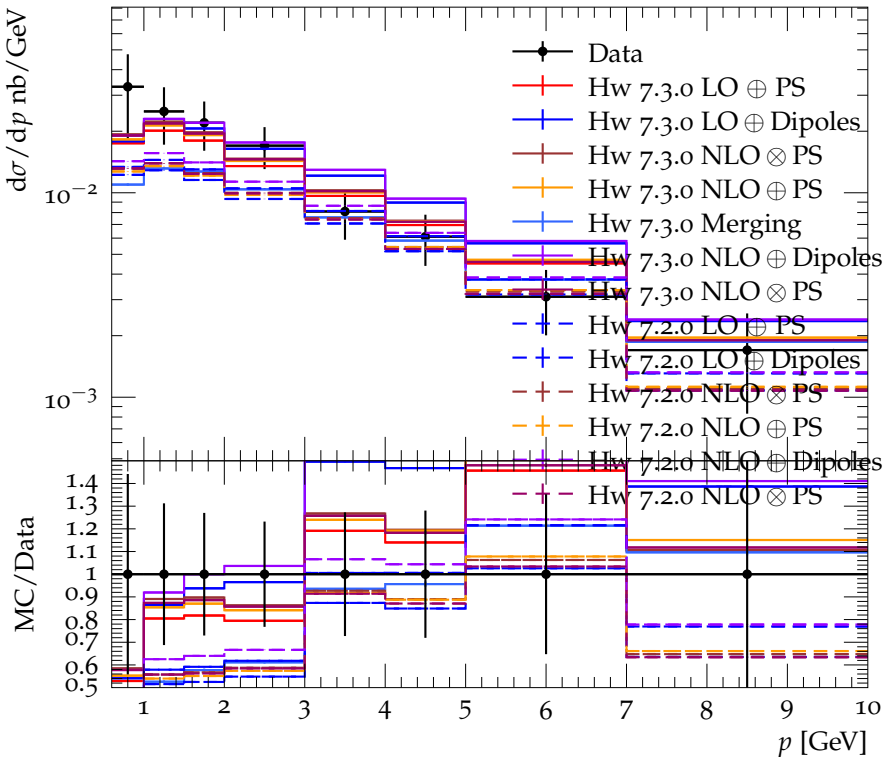
\Lambda^0, \bar{\Lambda}^0 momentum spectrum for E_{\text{CMS}} = 34 GeV
