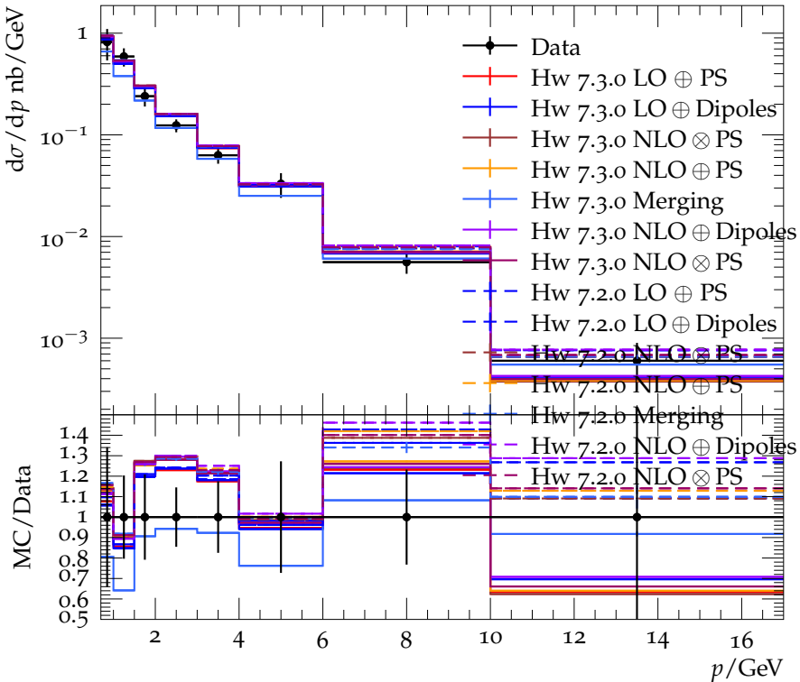
\pi^0 momentum spectrum for E_{\text{CMS}} = 34 GeV
