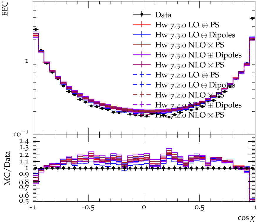
Energy-energy correlation, EEC for E_{\text{CMS}} = 14 GeV
