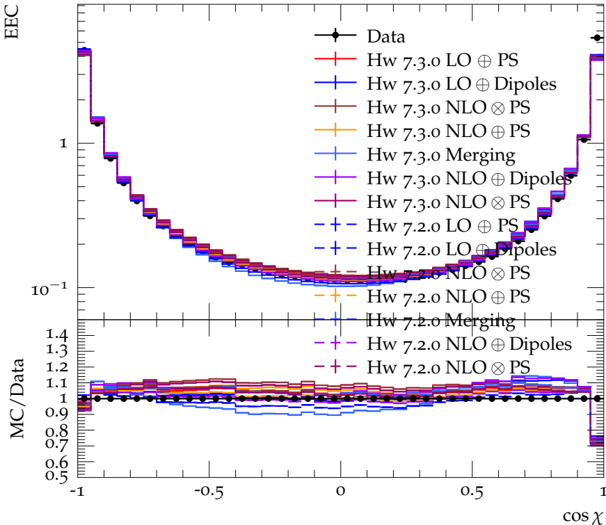
Energy-energy correlation, EEC for E_{\text{CMS}} = 34.8 GeV
