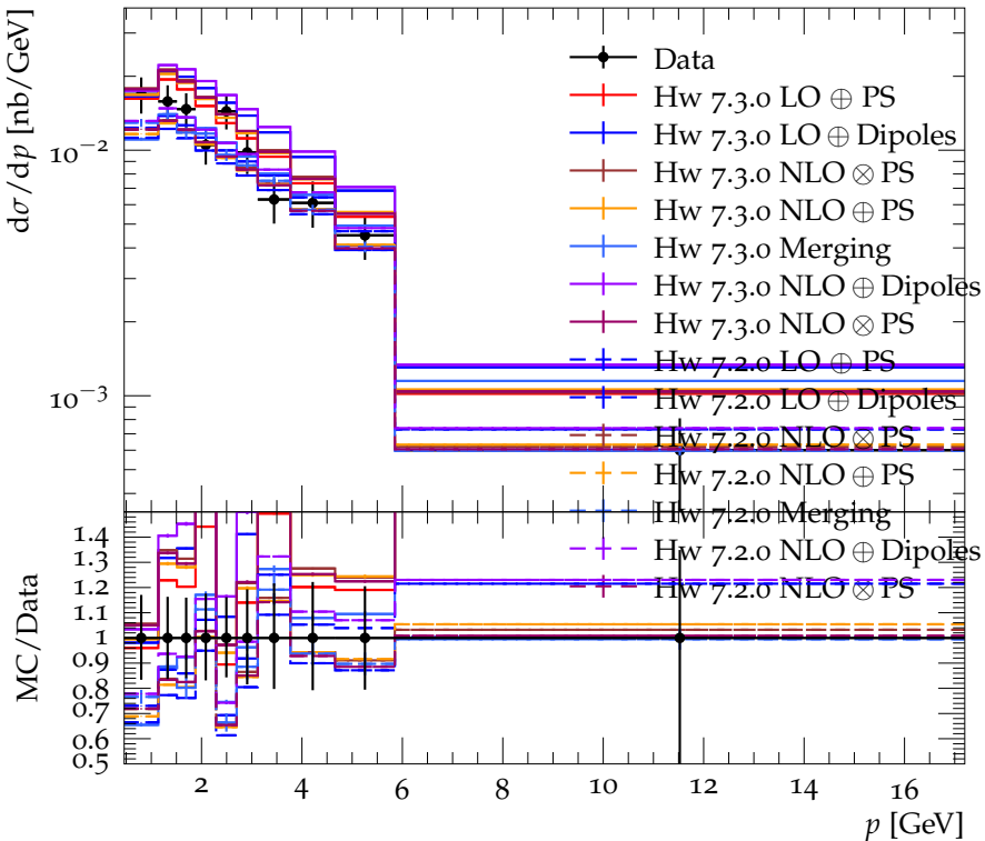
Momentum Spectrum for \Lambda^0, \bar{\Lambda}^0 at 34.8 GeV
