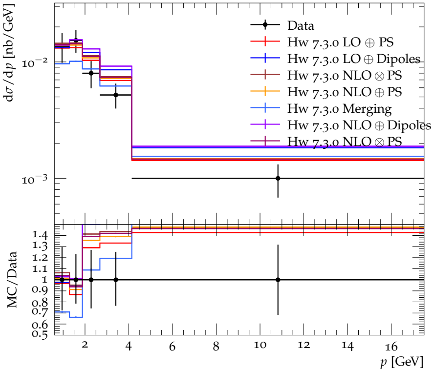
Momentum Spectrum for \Lambda^0, \bar{\Lambda}^0 at 42.1 GeV
