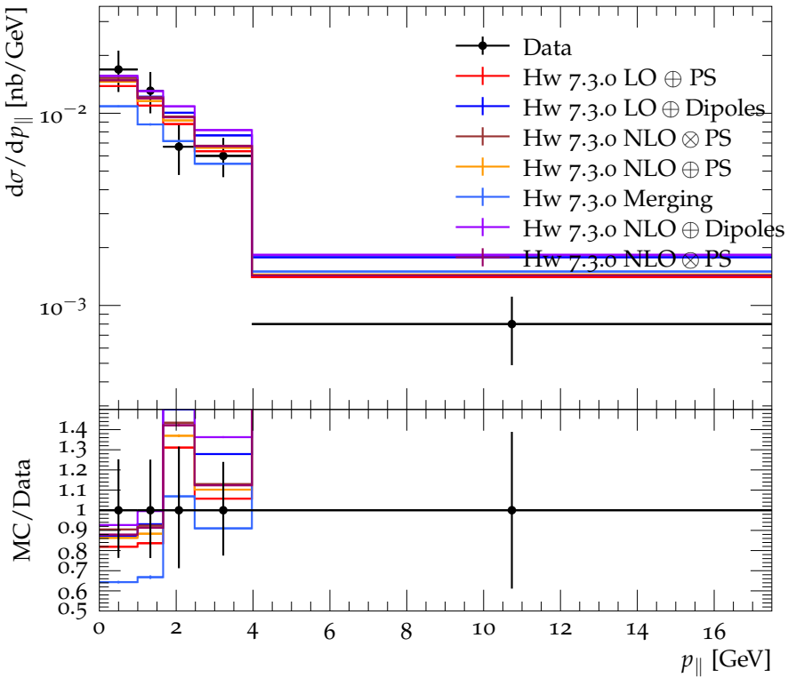
Momentum parallel to sphericity axis for \Lambda^0, \bar{\Lambda}^0 at 42.1 GeV
