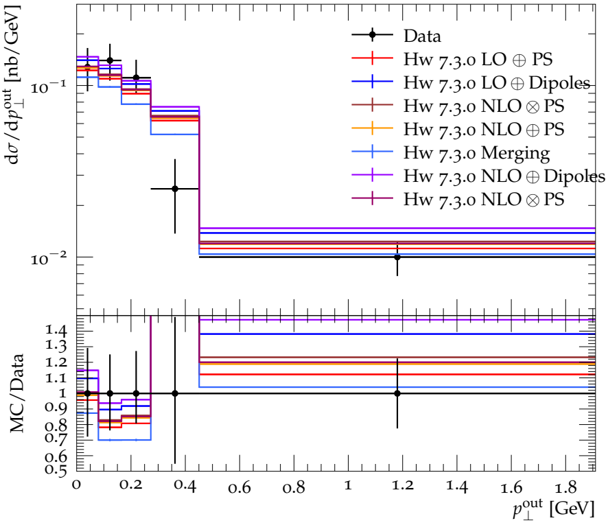
Out-plane momentum \perp to sphericity axis for \Lambda^0, \bar{\Lambda}^0 at 42.1 GeV
