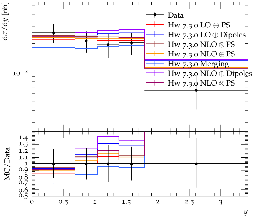
Rapidity w.r.t to sphericity axis for \Lambda^0, \bar{\Lambda}^0 at 42.1 GeV
