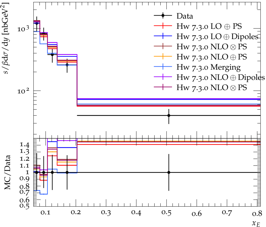
Scaled energy for \Lambda^0, \bar{\Lambda}^0 at 42.1 GeV
