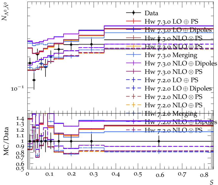
\Lambda^0, \bar{\Lambda}^0 multiplicity vs sphericity at 34.8 GeV
