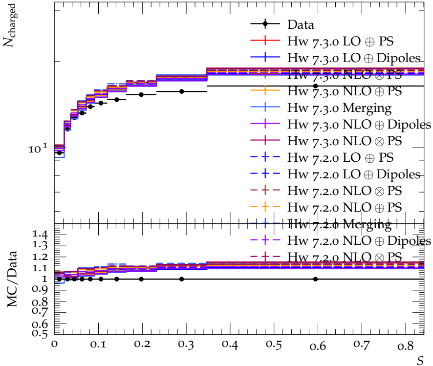
N_{\text{charged}} vs sphericity at 34.8 GeV
