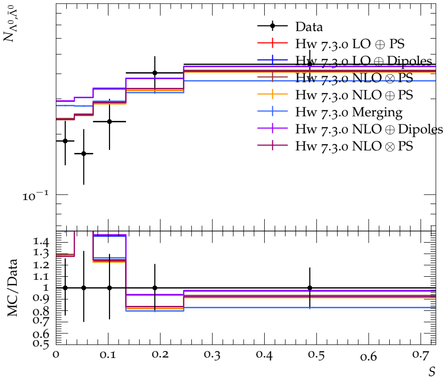
\Lambda^0, \bar{\Lambda}^0 multiplicity vs sphericity at 42.1 GeV
