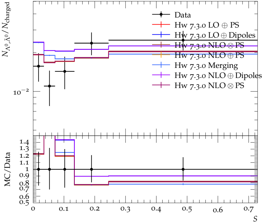
N_{\Lambda^0, \bar{\Lambda}^0} / N_{\text{charged}} vs sphericity at 42.1 GeV
