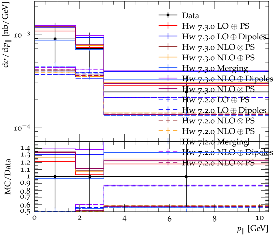
Momentum parallel to sphericity axis for \Xi^- , \Xi^+ at 34.8 GeV
