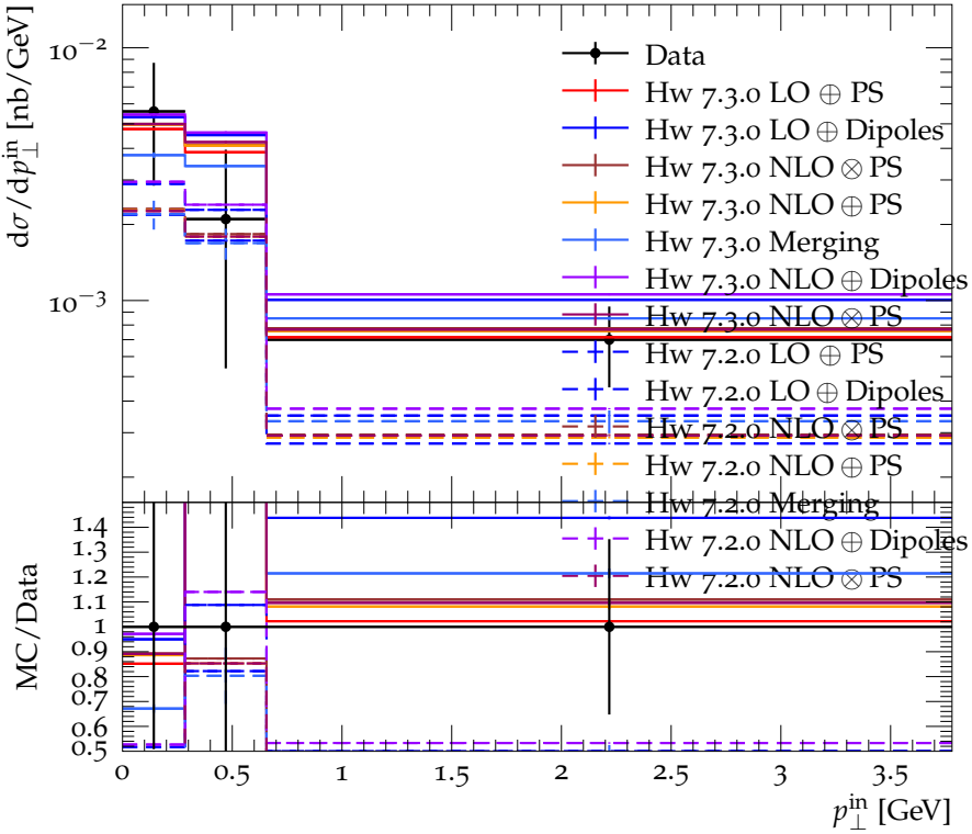
In-plane momentum \perp to sphericity axis for \Xi^- , \Xi^+ at 34.8 GeV
