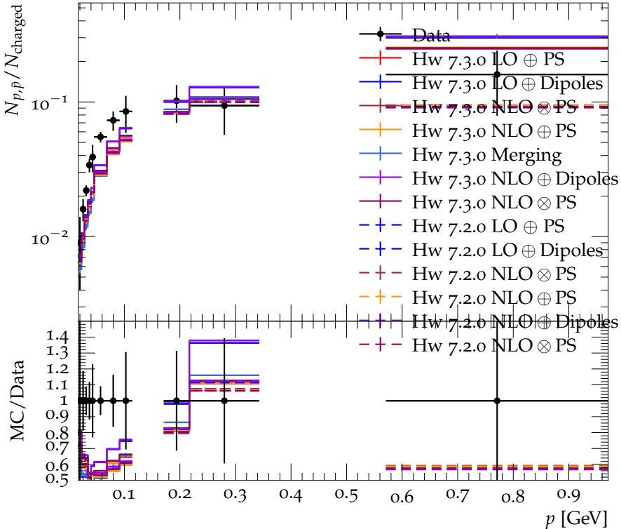
Ratio of p, \bar{p} to charged particles at 34 GeV
