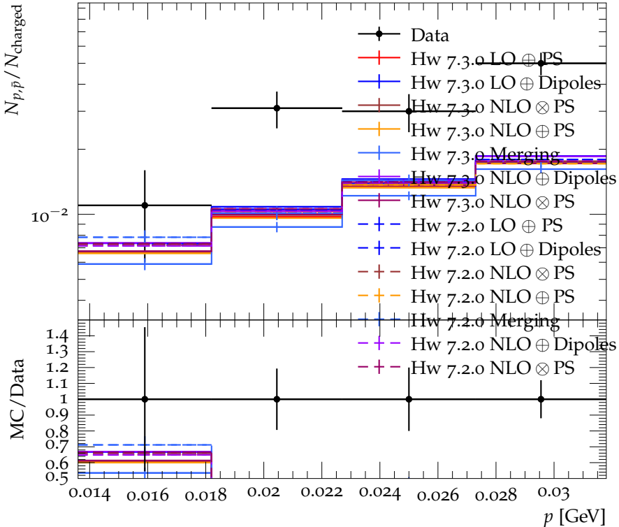
Ratio of p, \bar{p} to charged particles at 44 GeV
