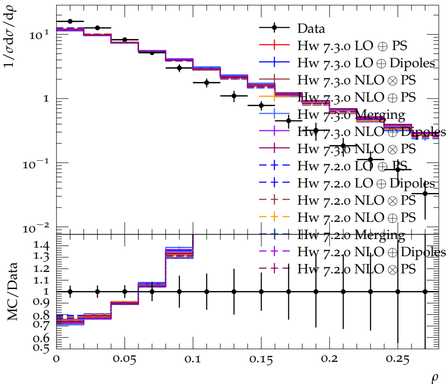
Scaled jet mass difference at 22 GeV
